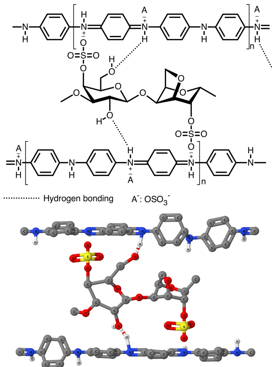
Fig. 4. Model of interaction \iota -CGN–PAni, indicating both ionic interaction \text{HN}^+ \cdots \text{OSO}_3^- and hydrogen bond interaction \text{O} \cdots \text{H}-\text{N}^+ .
